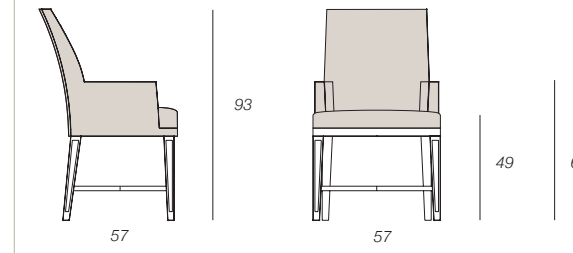
Poltroncina imbottita Upholstered armchair Gepolsterter Armstuhl
